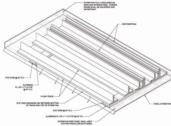
2 FLUSH TRACK & WEATHERTRAK - ISOMETRIC VIEW SCALE: 8" = 1'-0"
