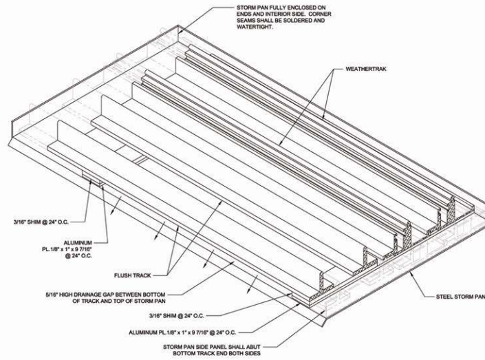
2 FLUSH TRACK & WEATHERTRAK - ISOMETRIC VIEW SCALE: 8" = 1'-0"
