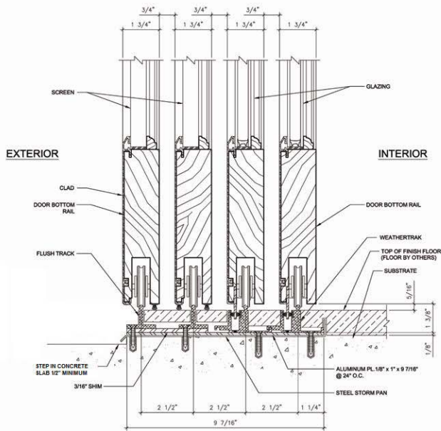
1 FLUSH TRACK & WEATHERTRAK - 4 TRACK SYSTEM SCALE: 8" = 1'-0"
