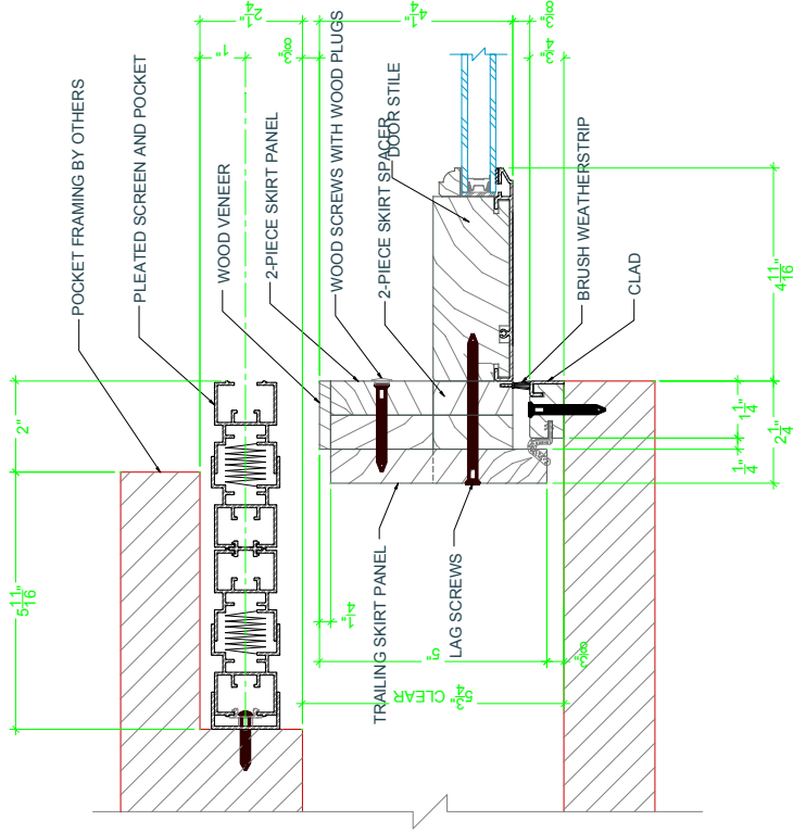
TYPICAL 2 - PANEL POCKET
