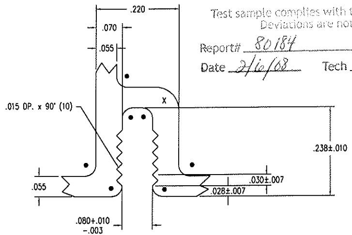
DETAIL "B"
