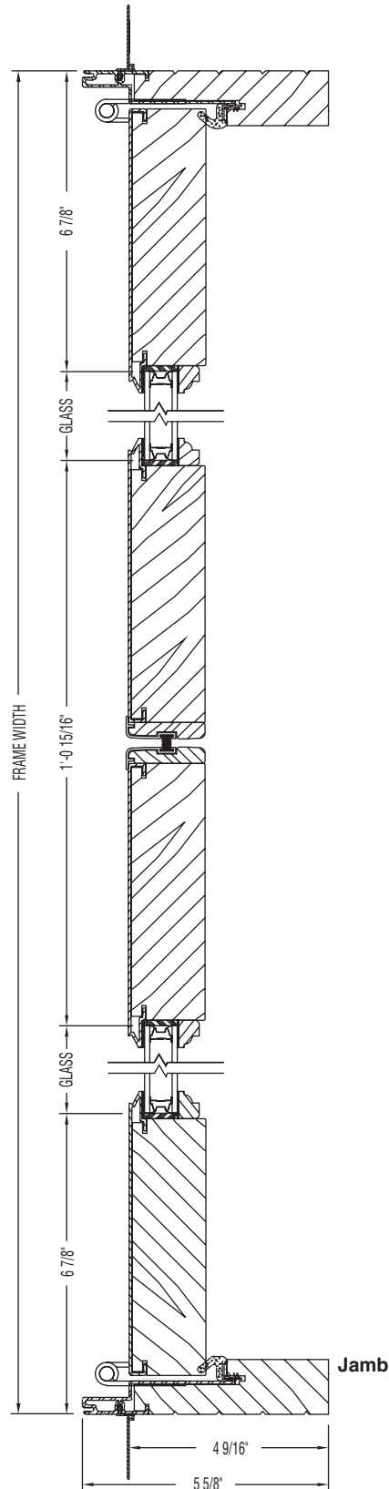
Double French Commercial Door — CP2
