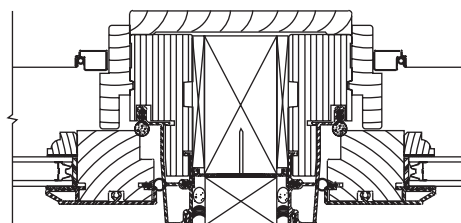
2" Mullion (Field Application)
