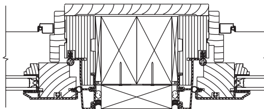
3 1/2" Mullion (Field Application)
