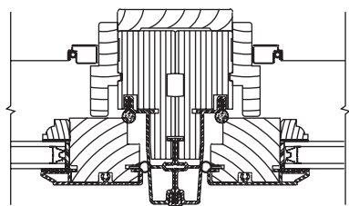
Standard Mullion
