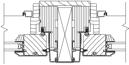
1" Mullion
