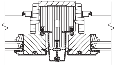
Standard Mullion
