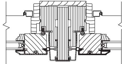
3/4" Mullion
